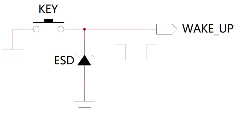
Figure 9: Key reset reference circuit
